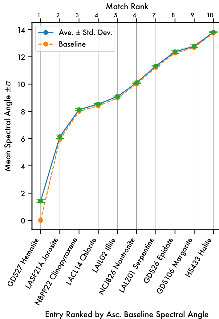
GDS27 Hematite Mean Spectral Angle Match
